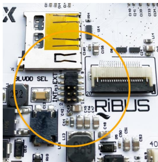
Figure 6. External backlight jumper setting
