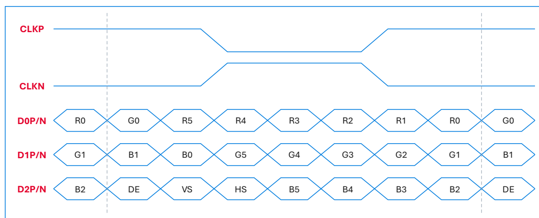
6-bit RGB LVDS input timing
