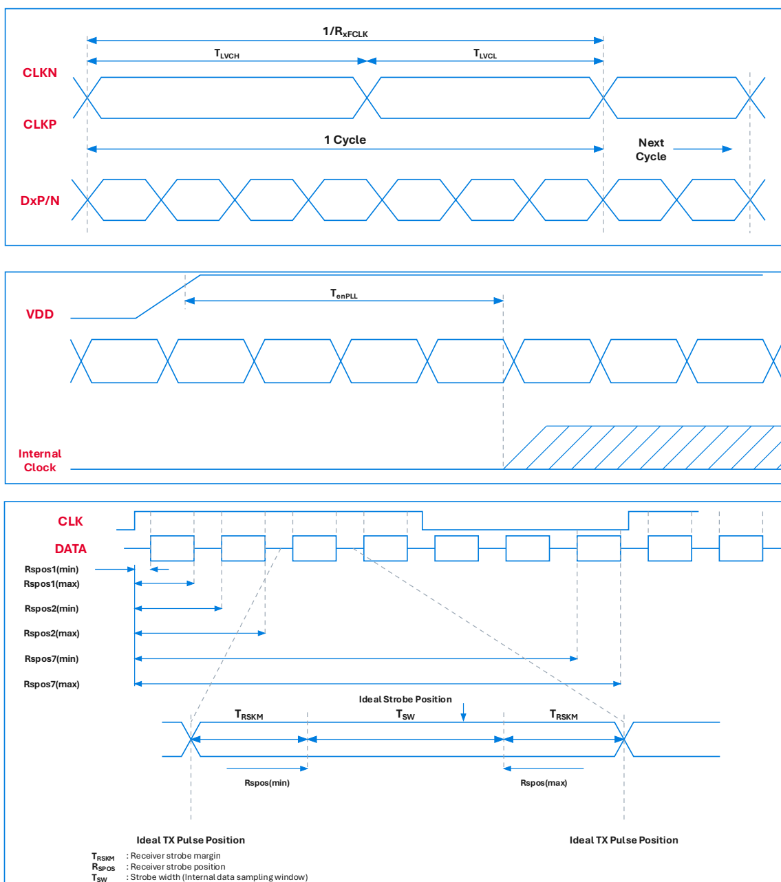
LVDS figure
