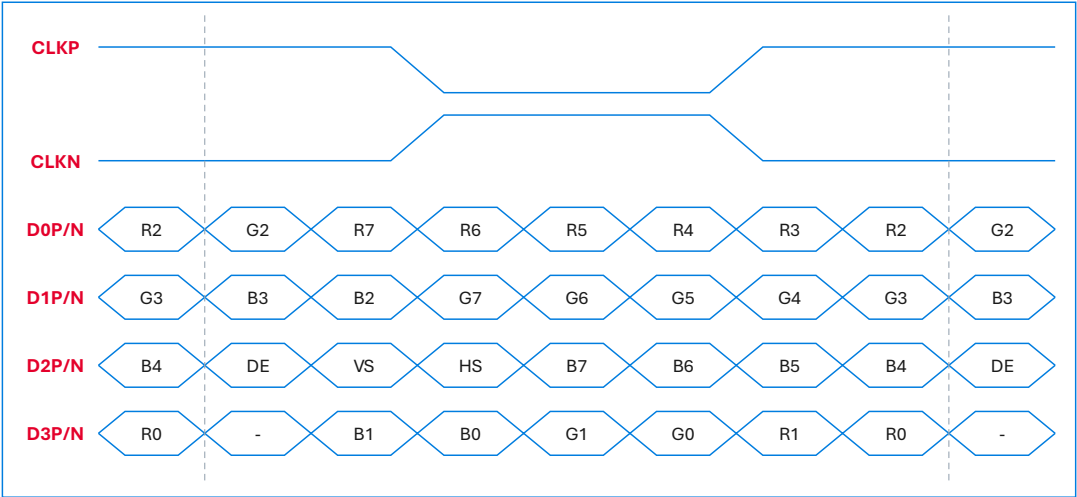
8-bit RGB LVDS JEIDA input timing
