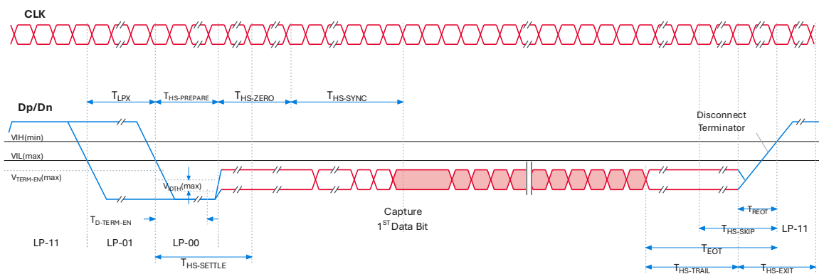
Timing of high-speed data transmission in bursts
