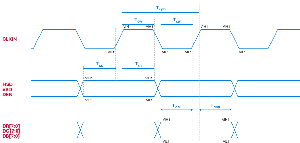
Input signal timing
