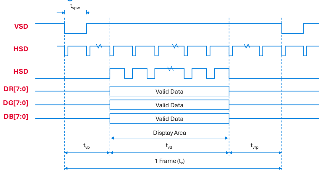
24-bit parallel RGB mode horizontal/vertical input timing
