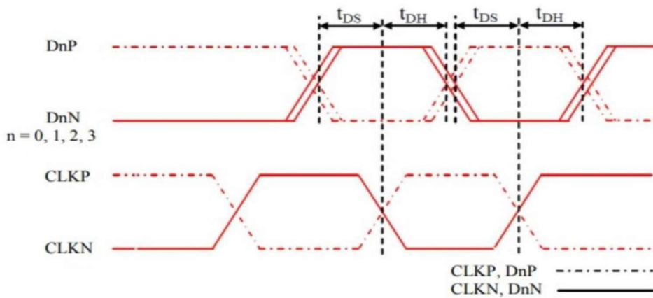
Figure 2 Data to Clock Channel Timing
