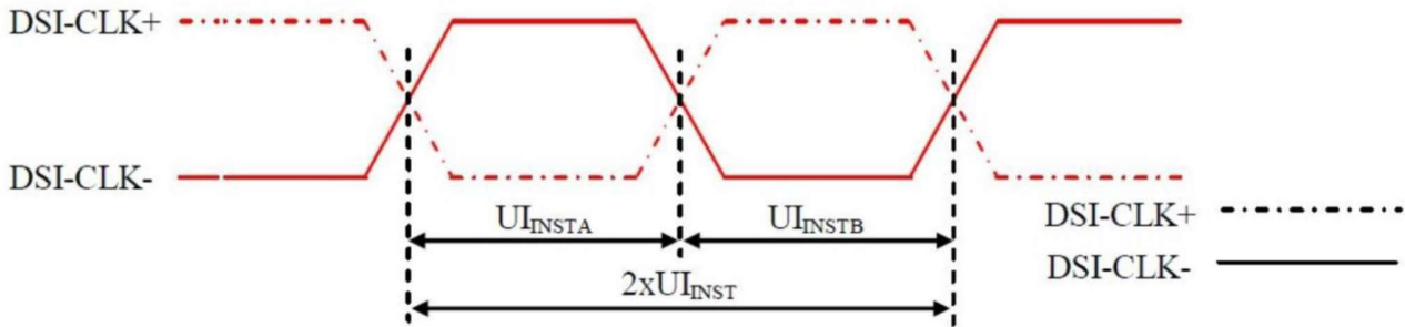
Figure 1 DSI Clock Channel Timing
